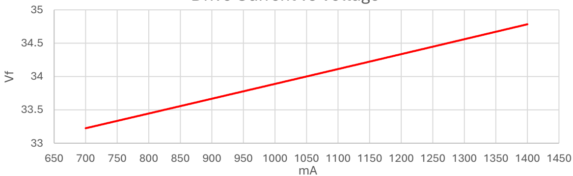
Drive Current vs Voltage
