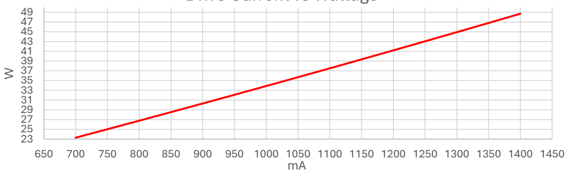
Drive Current vs Wattage
