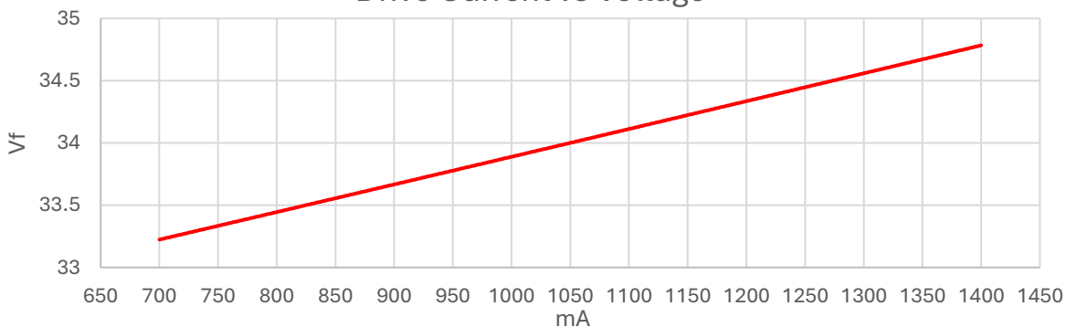
Drive Current vs Voltage
