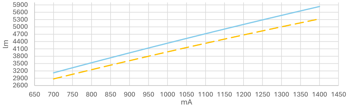
Drive Current vs Lumens
